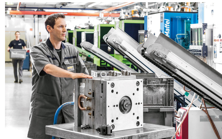
Injection molding
