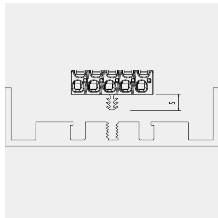
Extruded aluminium profile with M4 thread channel
