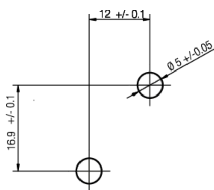
LBK 1/5 ST | Plate thickness: 0.4 mm
