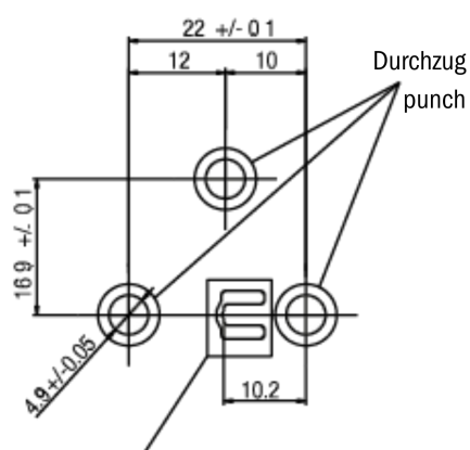
LBK 1/7 ST E-PIEC | Plate thickness: 0.4 mm
