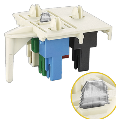
Push-in earth contact (without VDE)
