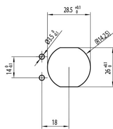
KADO 2/3 OZ OS | Plate thickness 0.5 – 1.0 mm | PH2 - 1,2 Nm
