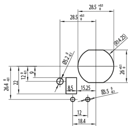
KADO 2/3 EE OS | Plate thickness 0.5 – 1.0 mm | PH2 - 1,2 Nm
