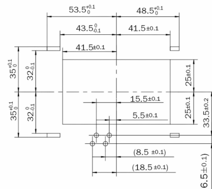
Cutout four-hole-earth-tag | Plate thickness 0.5 - 1 mm
