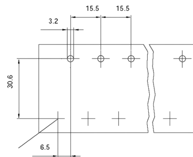
Cutout | Position for earth cutout
