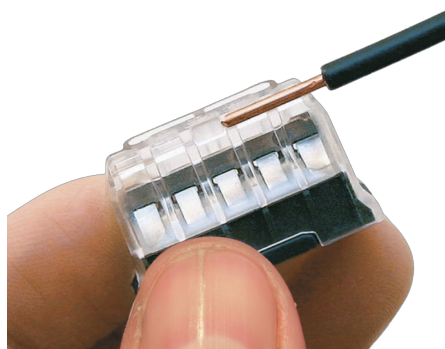
Gauge wire stripping length
